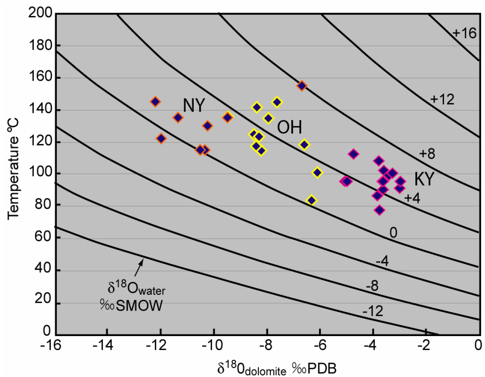
Figure 63. Data from New York, Ohio and Kentucky plotted on Figure 18. NY fluid looks like it was a bit lighter ( \sim +2\text{‰} ) than the fluid in KY and OH (around +4 or +5\text{‰} ).
