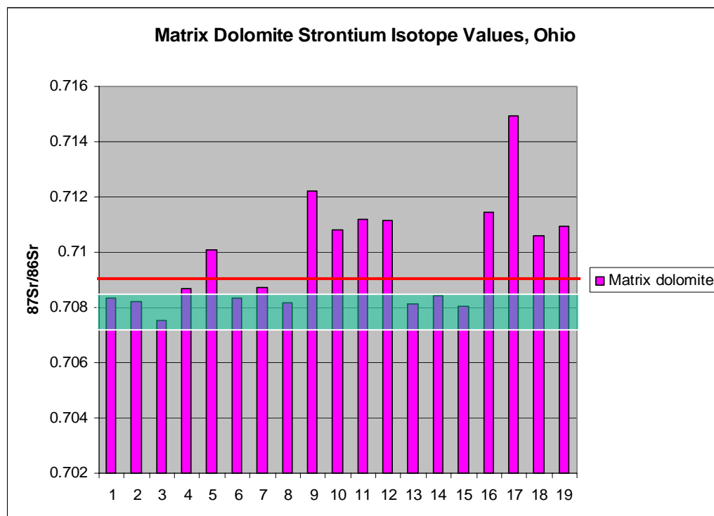
Figure 67. Strontium isotope ratios for matrix dolomite in Ohio samples. About half the samples fall within the seawater range and half exceed it.
