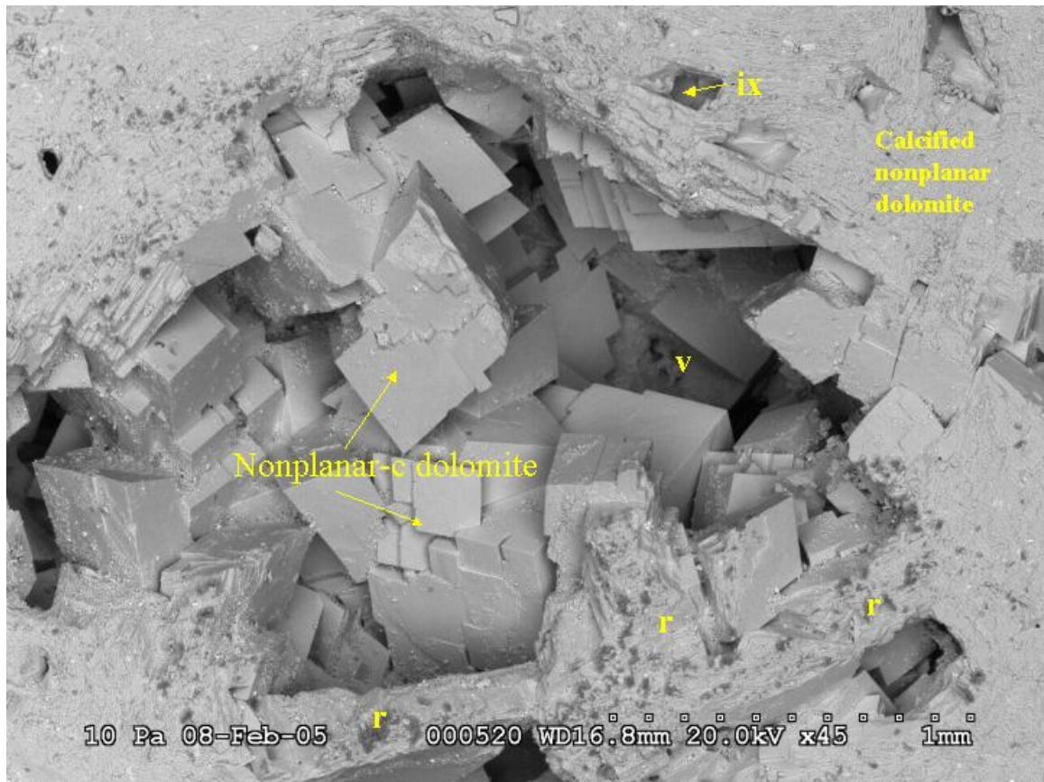
Figure 34. Backscattered electron (BSE) image obtained by scanning electron microscopy (SEM) of the dolograine shown above in figures 31A and 34. The small vug (v), about 2.5 mm across, formed through dissolution of calcified nonplanar dolomite (see Figure 36 below). Note the remnant (r) of the latter near the bottom of the void. The vug is partially filled with nonplanar-c (saddle) dolomite. Some of these crystals are also corroded due to dissolution. Some small (<0.1 to 0.2 mm) intracrystalline voids occur in this sample.
