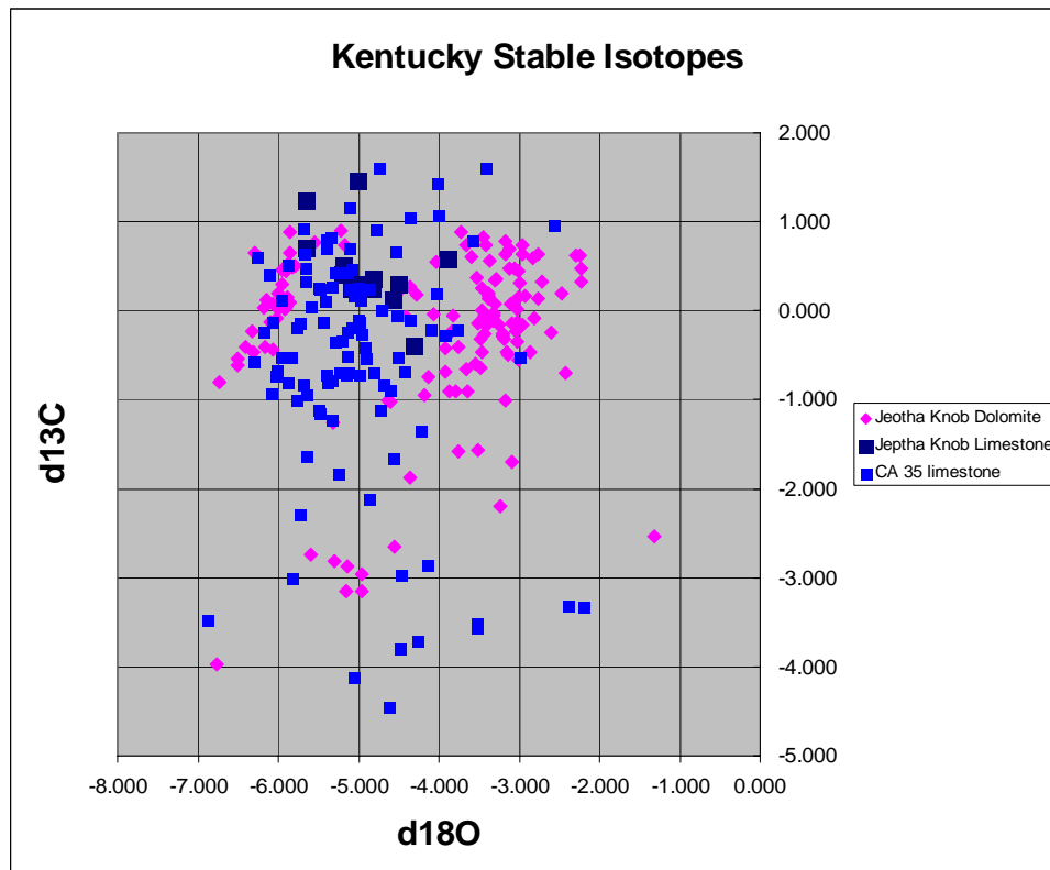
Figure 61. Stable isotope values from Kentucky Jeoptha Knob dolomites and limestones.
