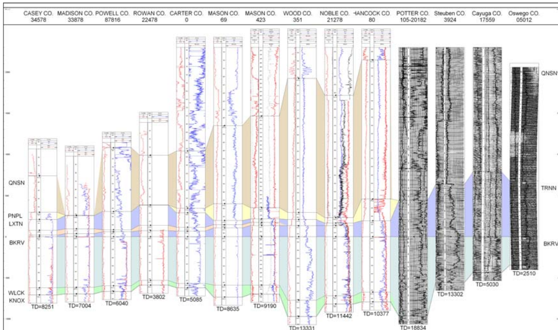
Figure 27. Regional stratigraphic strike cross section D-D' from Kentucky to New York illustrating the Cambrian-Ordovician units.
