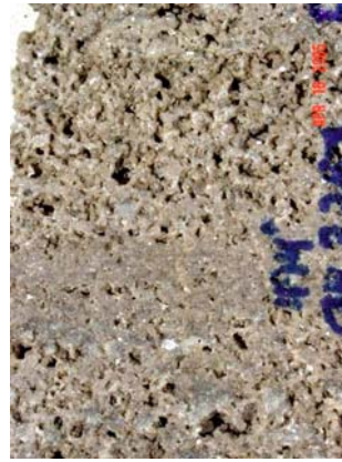
Figure 31. Dolograins from Trenton Group reservoirs in northwest Ohio. A. Dolograins with recognizable depositional texture. The rock consists of cross-bedded, coarse-grained crinoid-bryozoan grainstone interbedded with stylolitic dolomudstone/dolowackestone. These cyclic lithologies consist of shoaling-upward, grainstone-capped subtidal parasequences. Note the large crinoid allochem, which is mimetic planar-s to nonplanar-a (transitional) dolomite (also see Figure 32). The visible porosity consists mostly of small vugs, 0.5 to 4 mm in diameter, and molds. (OH 3479, Hancock Co., Palladin Enterprises, Anderson well, 1337.8 ft.). B. Interpreted dolograins without recognizable depositional texture. Dolomitization has obliterated all of this rock's primary and earlier diagenetic fabrics. The interpretation of this sample as a former grainstone is based on the presence of allochem ghosts, and both mimetic and non-mimetic replacement textures observed in thin section (Figure 33). (OH 3267, Auglaize Co. Meridian, Bousher #1 well, 1174 ft.).
