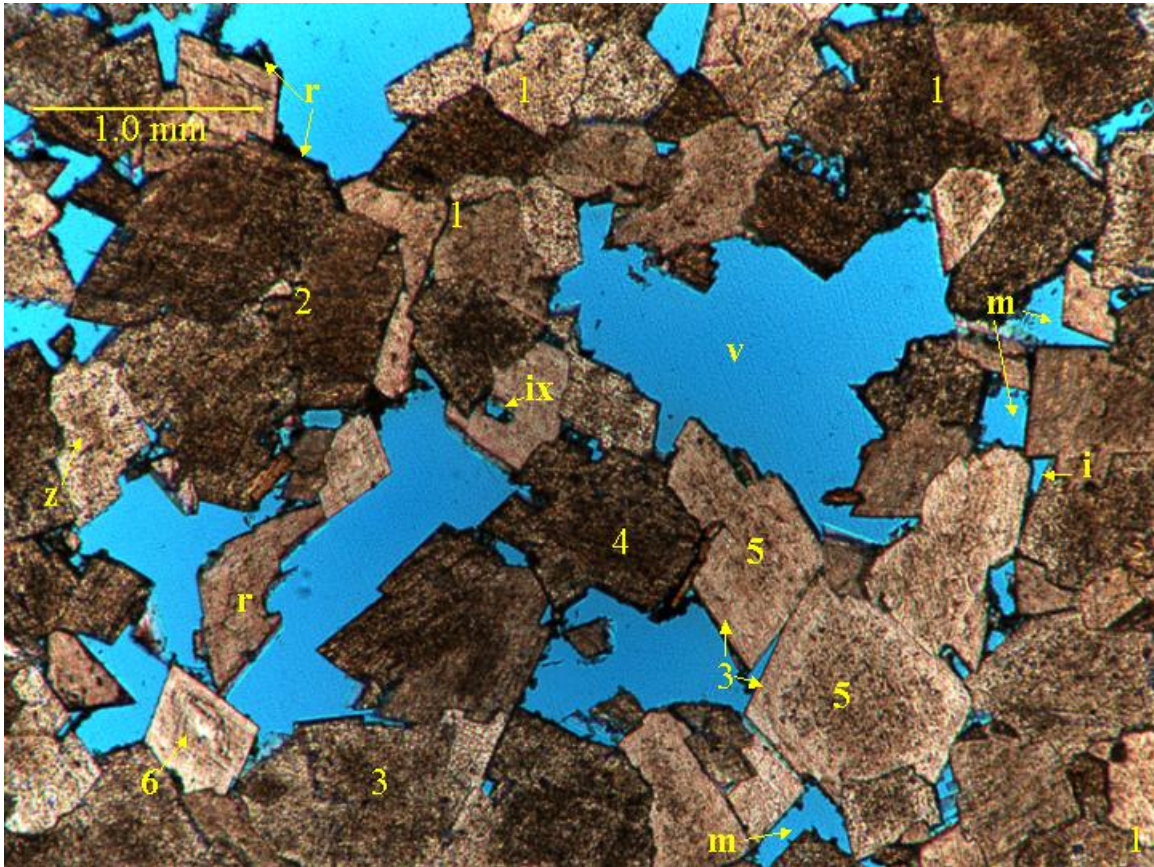
Figure 33. Dolomite texture and porosity in dolograine reservoir rocks, northwest Ohio. This is a photomicrograph (plane polarized light) of a dolostone with recognizable depositional texture (same sample shown in Figure 31A). The sample is polymodal, coarsely to very coarsely crystalline dolostone. Crystal size ranges from 0.1 to 1.2 mm, with a mean of 0.6 mm. The rock consists of (1) planar-s to nonplanar-a (transitional) dolomite, (2) nonplanar (saddle) dolomite, and (3) nonplanar-c dolomite. About 25 percent of the dolomite crystals present in the rock partially to wholly take a stain with Alizarin Red S indicating partial calcification of the dolostone (4). Cloudy cores of planar-e and planar-s dolomite, revealed by inclusion patterns incorporated in the dolomite crystals, have overgrowths of nonplanar-c or saddle dolomite cement (5). Relicts or ghosts of zoned crystal growth can be discerned in some crystals (6). Mesopores (intercrystalline, i, moldic, m, and intracrystalline, ix) are fabric selective. Macropores consist of small vugs 0.5 to 4mm in diameter (v). Partial to almost complete dissolution of calcified dolomite crystals created the macropores (small vugs). Note the remnants and residues of partially to completely calcite-replaced dolomite (r). Dissolution of dolomite resulted in some of the moldic voids.
