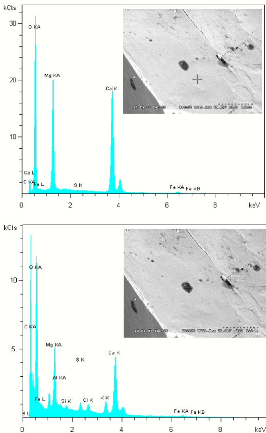
Figure 35. Hydrocarbon stains on nonplanar-c dolomite (saddle dolomite cement). A. SEM and energy dispersive x-ray spectroscopy (EDS) of cement crystals in dolograinstone. The cross shows the location of the EDS analysis of the crystal, which is clearly dolomite. B. EDS analysis of the black stain on the dolomite crystal reveals its high carbon concentration relative to the Mg and Ca of the dolomite itself. (OH 2549, Wood Co., 1168.25 ft.)
